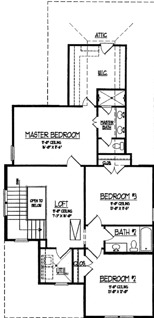
SECOND LEVEL FLOOR PLAN
