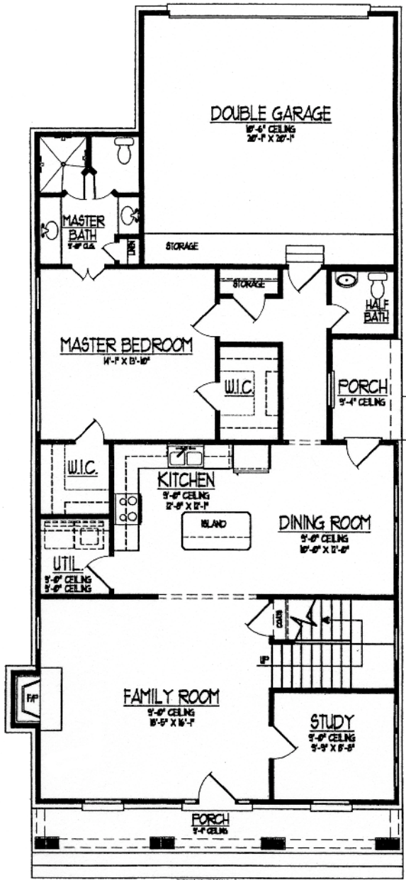
FIRST LEVEL FLOOR PLAN
