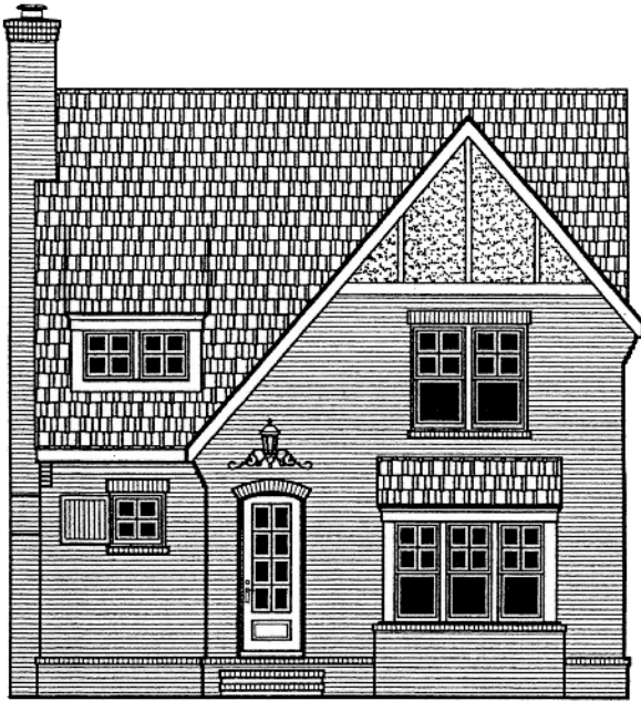
FRONT ELEVATION
