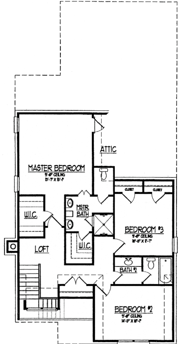
SECOND LEVEL FLOOR PLAN
