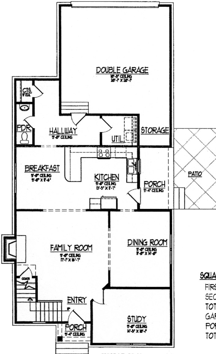
FIRST LEVEL FLOOR PLAN
